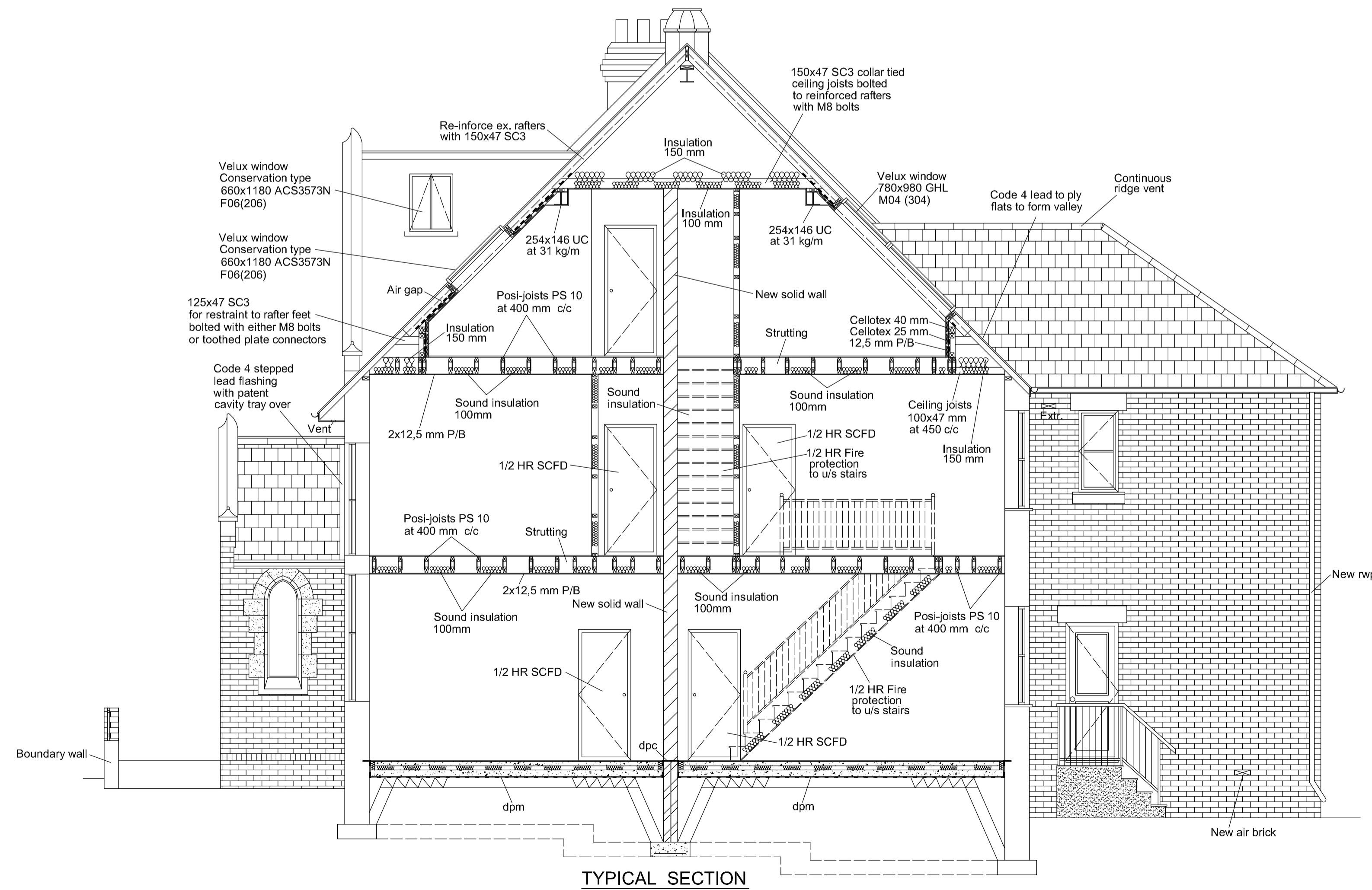
TYPICAL SECTION
